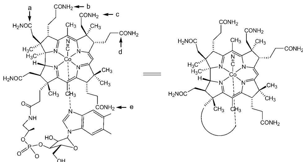
Scheme 1. Assignment of the side chains on the periphery of the corrin ring in B 12 .
