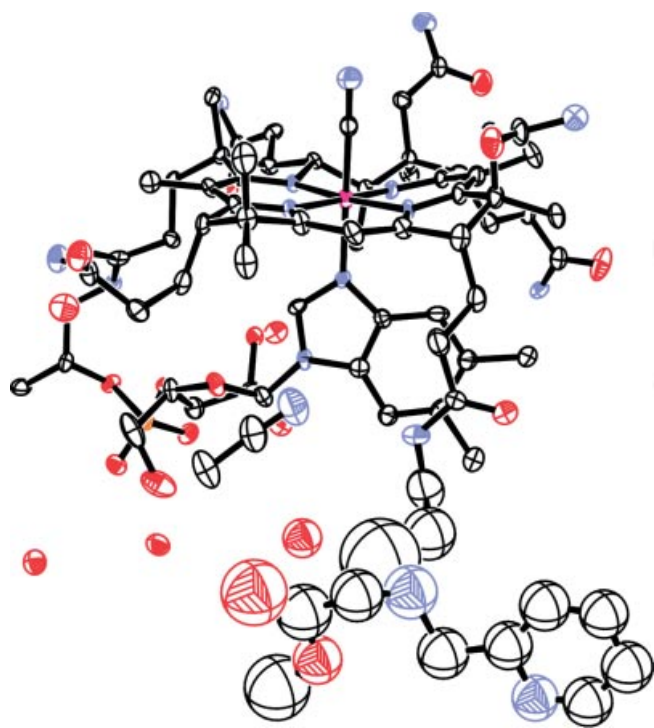
Figure 3. ORTEP plot of 5 . Hydrogen atoms and some water molecules were omitted for clarity.
