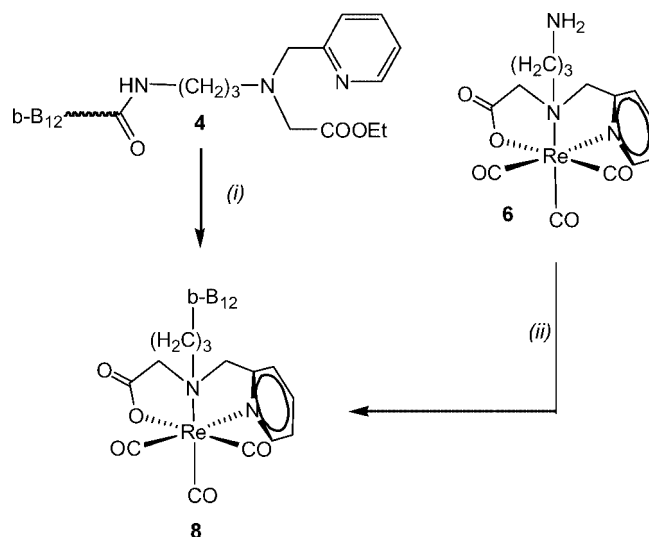
Scheme 4. Reaction pathways to 8 , (i) direct reaction of 4 with [Re(OH_2)_3(CO)_3]^+ to give 8 (postlabelling) or (ii) conjugation of preformed 6 to 1 (prelabelling).
