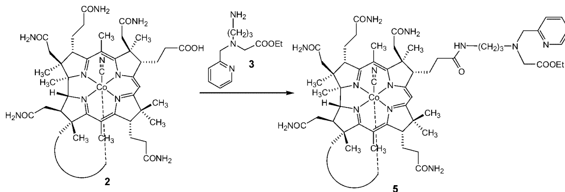
Scheme 3. Derivatisation of B 12 d-acid 2 with ligand 3 to yield compound 5 .
