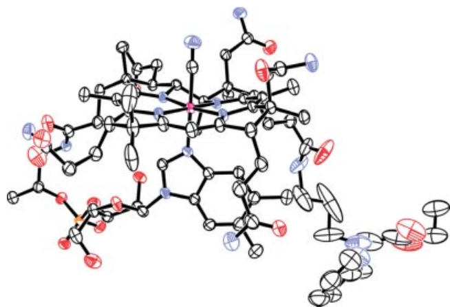
Figure 2. ORTEP plot of 4 . Hydrogen atoms and some water molecules were omitted for clarity.
