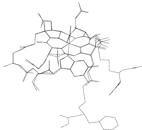
Figure 1. Overlay of the X-ray structures of 4 and 5 .
