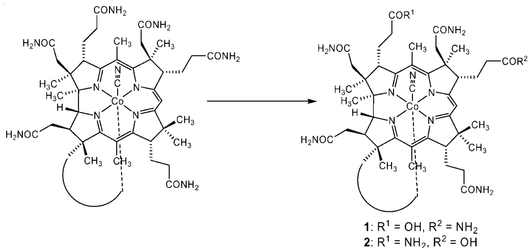
Scheme 2. Mild hydrolysis of B 12 yields the b- and d-acids 1 and 2 . [8,25–27]
